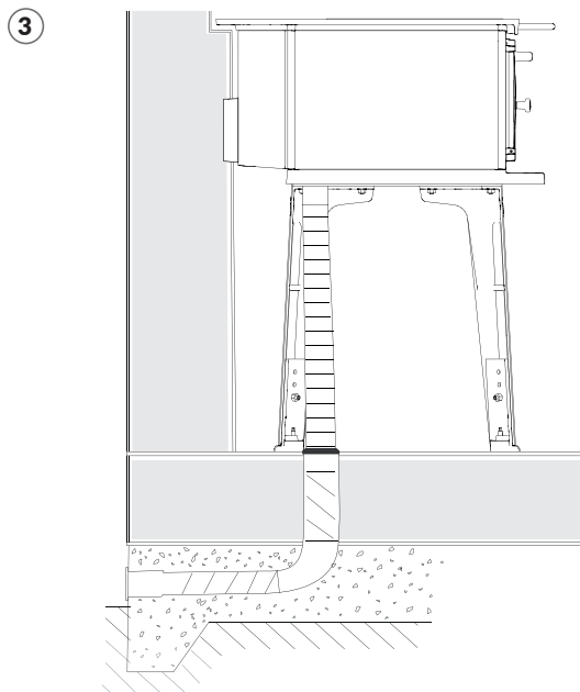
Connection to outdoor air via bottom plate. To be used primarily for new-builds.
